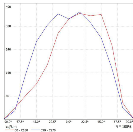
Illumination Curve
