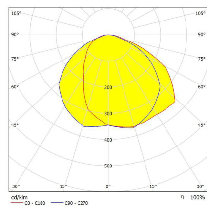
Luminance Distribution
