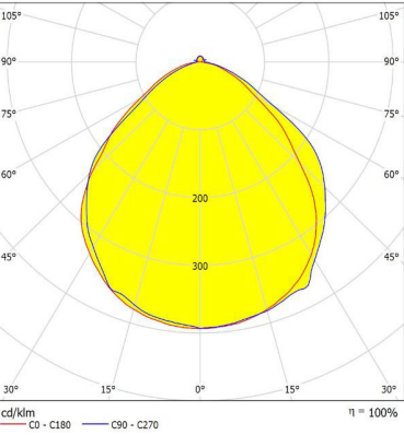
Luminance Distribution
