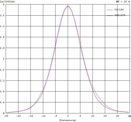
Illumination Curve
