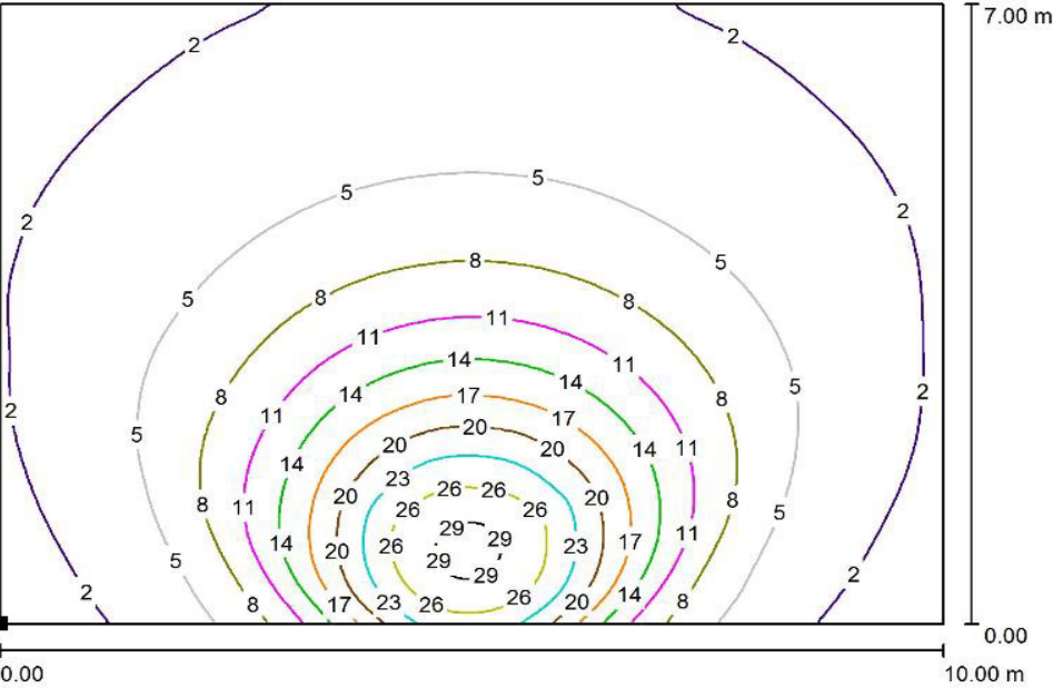
Illumination Curve
