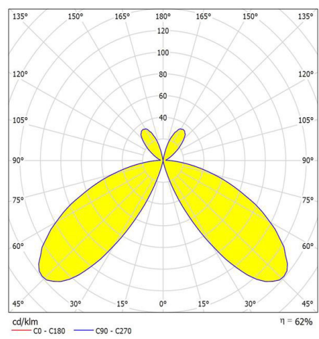
Illumination Curve
